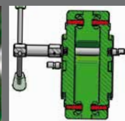
mounted carriage on 8 steel rolls, all adjust- ing elements with wrench size 19 mm
